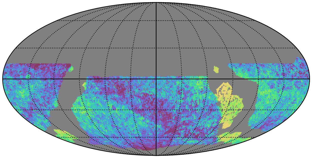
ddf_acor_sf10_lsf15_lsr10_v3.4_10yrs WFD all bands: Median skyBrightness
