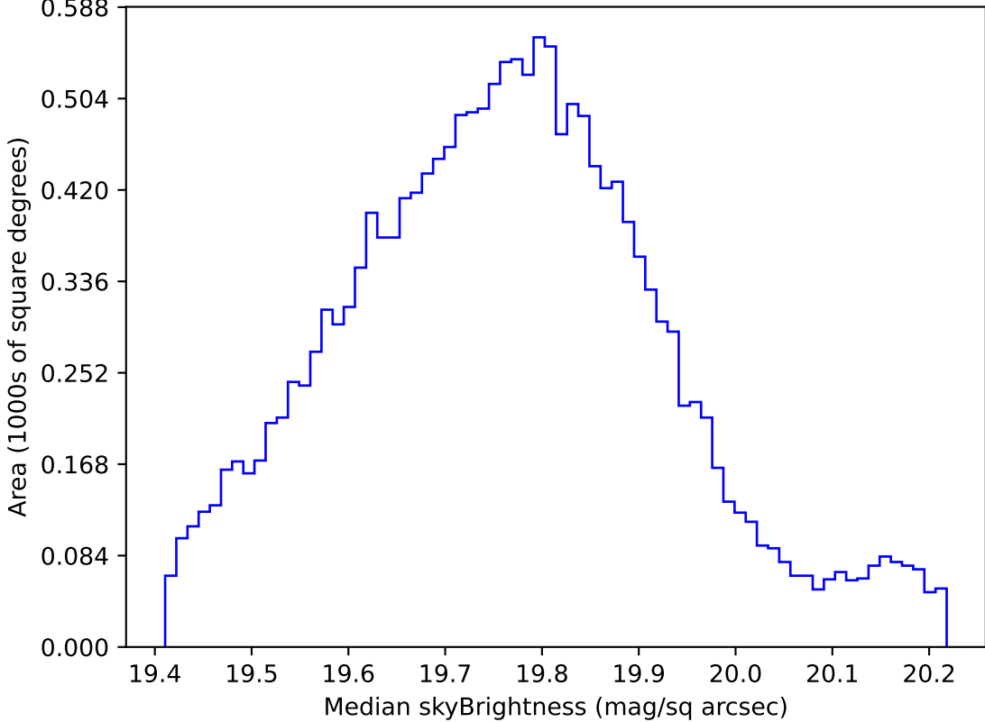
ddf_acor_sf10_lsf15_lsr10_v3.4_10yrs WFD all bands: Median skyBrightness
