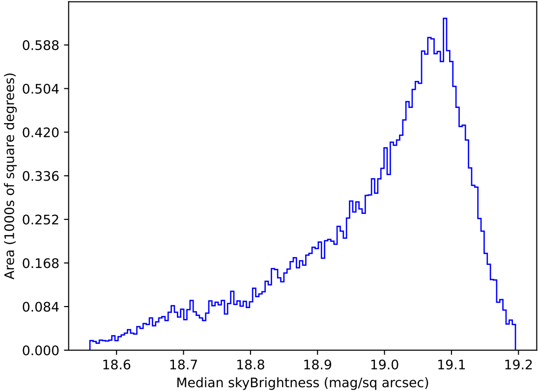
ddf_acor_sf10_lsf15_lsr10_v3.4_10yrs All sky z band: Median skyBrightness
