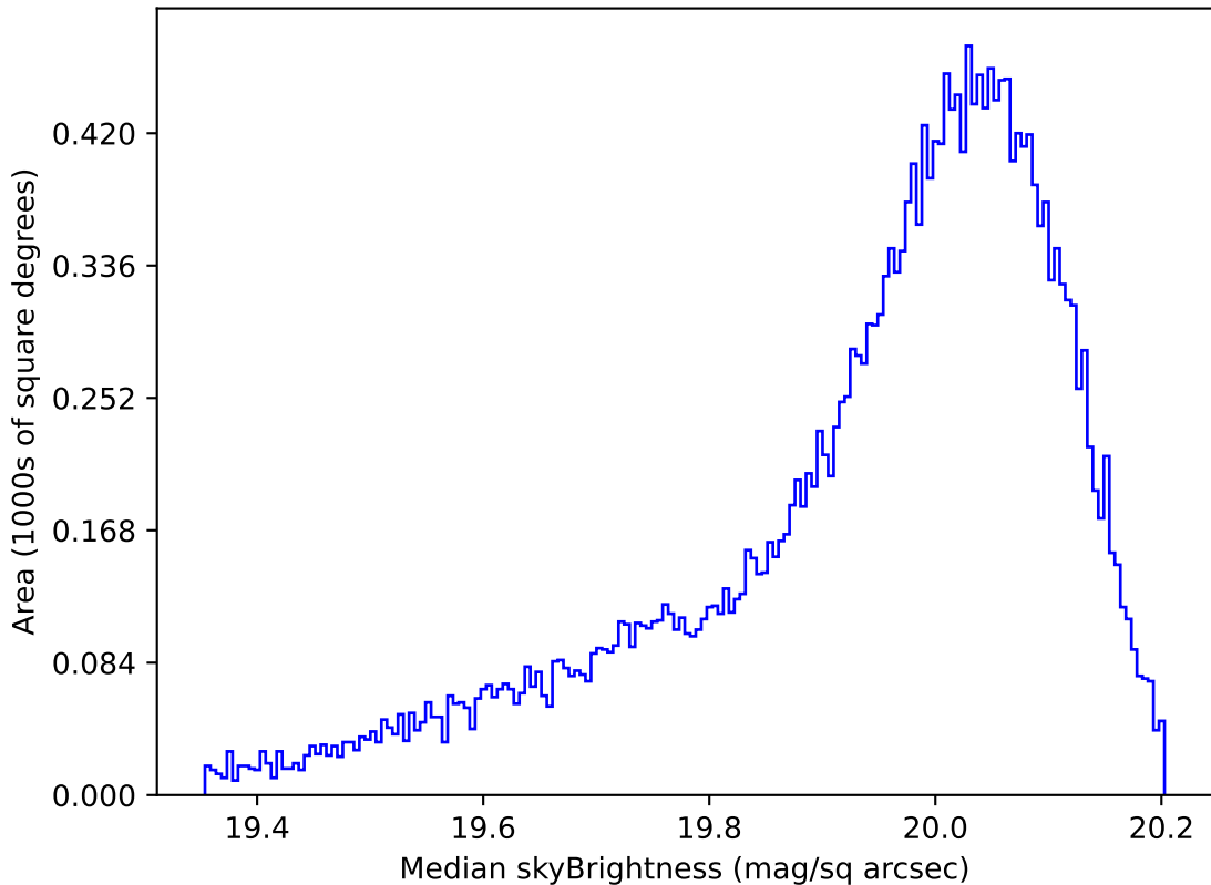
ddf_acor_sf10_lsf15_lsr10_v3.4_10yrs All sky i band: Median skyBrightness
