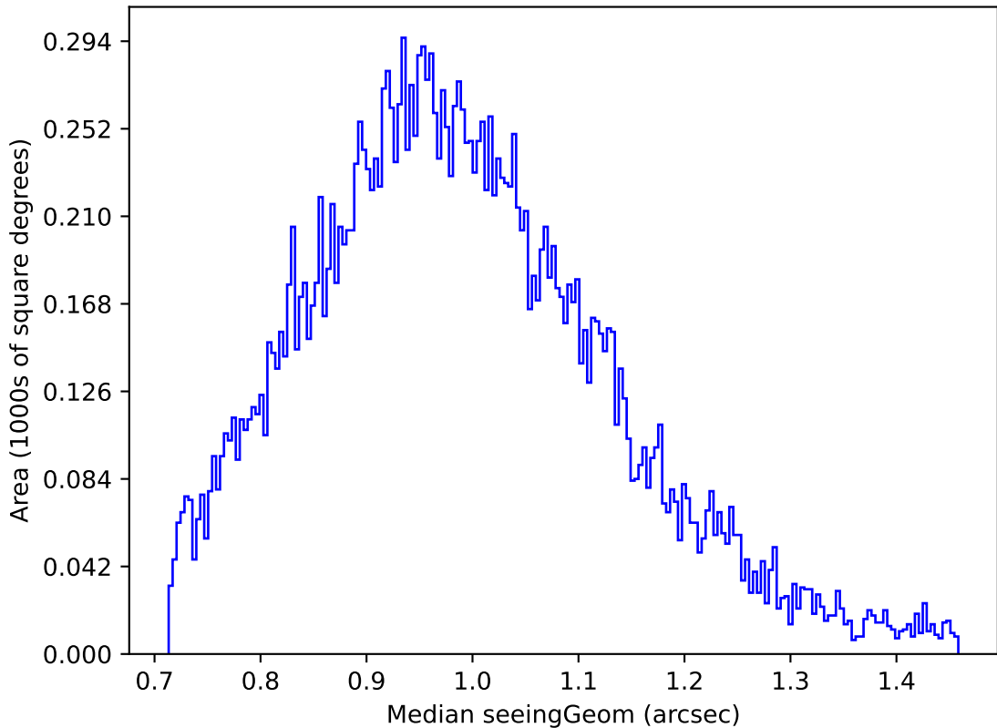
ddf_acor_sf10_lsf15_lsr10_v3.4_10yrs Yr 1 u band: Median seeingGeom
