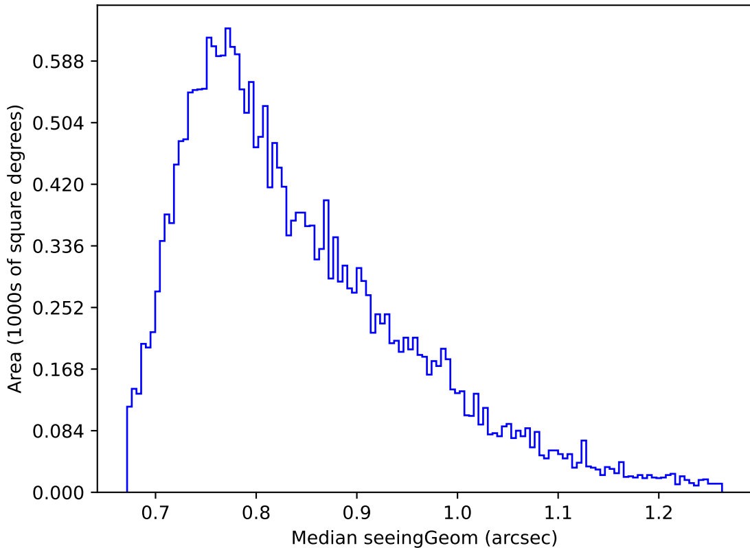
ddf_acor_sf10_lsf15_lsr10_v3.4_10yrs Yr 1 i band: Median seeingGeom
