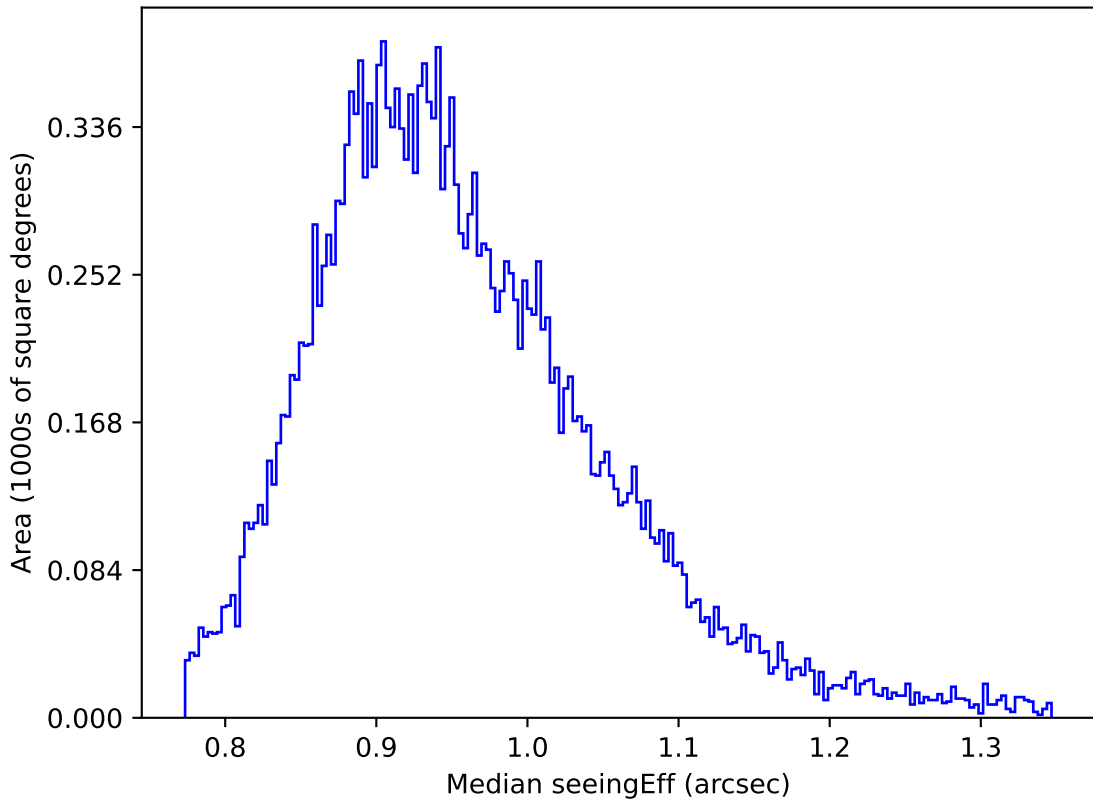
ddf_acor_sf10_lsf15_lsr10_v3.4_10yrs Yr 1 y band: Median seeingEff
