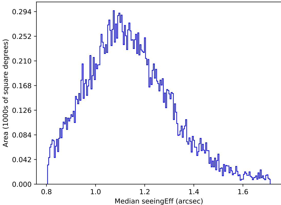
ddf_acor_sf10_lsf15_lsr10_v3.4_10yrs Yr 1 u band: Median seeingEff
