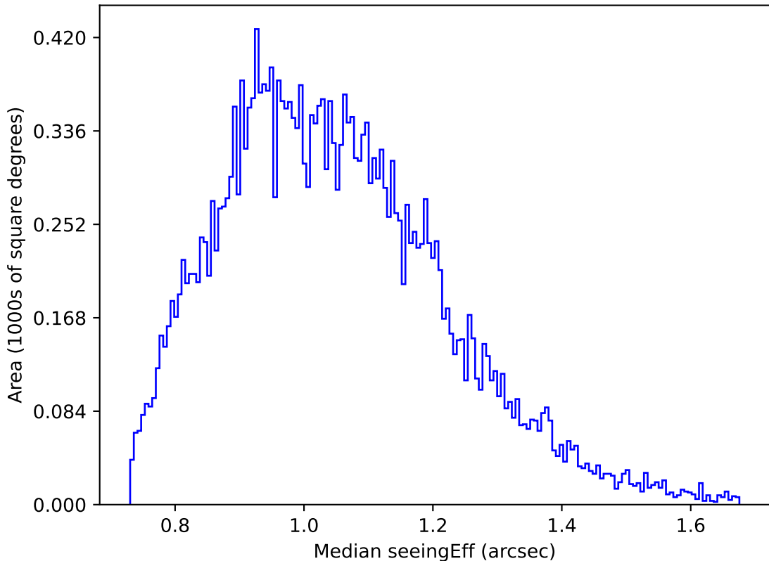
ddf_acor_sf10_lsf15_lsr10_v3.4_10yrs Yr 1 g band: Median seeingEff
