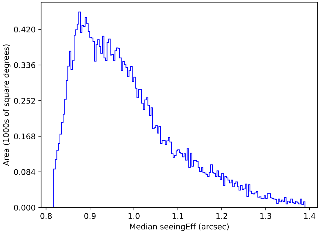
ddf_acor_sf10_lsf15_lsr10_v3.4_10yrs Yr 1 all bands: Median seeingEff
