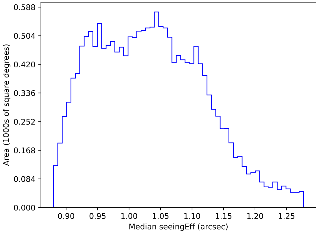
ddf_acor_sf10_lsf15_lsr10_v3.4_10yrs WFD r band: Median seeingEff
