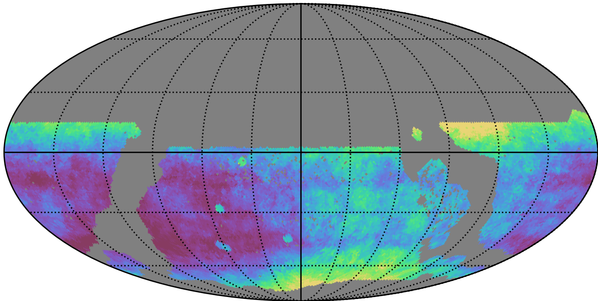
ddf_acor_sf10_lsf15_lsr10_v3.4_10yrs WFD i band: Median seeingEff
