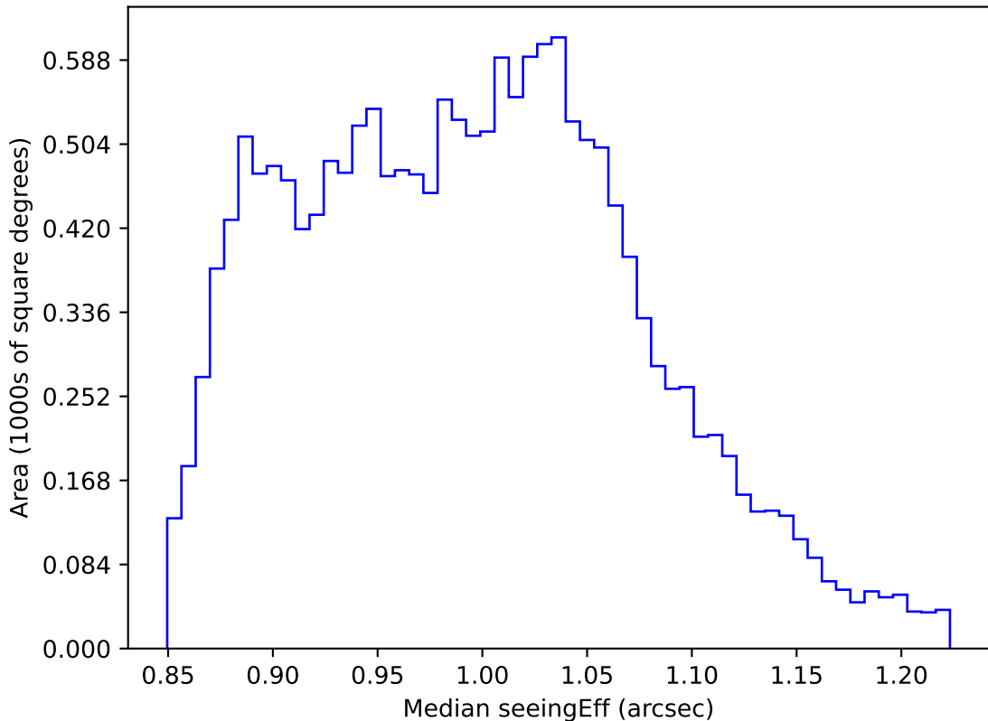
ddf_acor_sf10_lsf15_lsr10_v3.4_10yrs WFD i band: Median seeingEff
