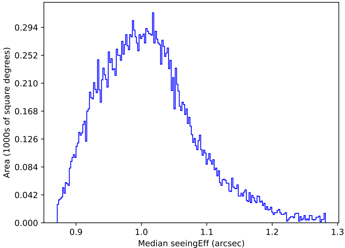
ddf_acor_sf10_ls15_lsr10_v3.4_10yrs All sky y band: Median seeingEff
