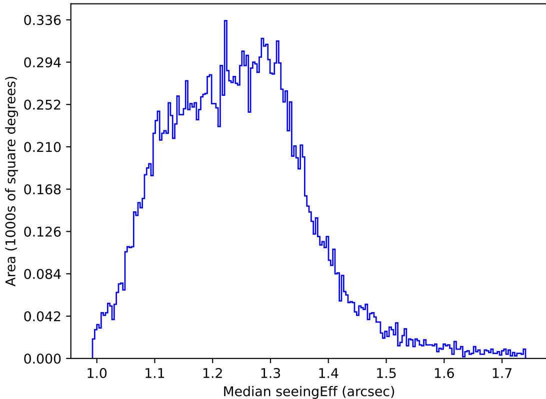
ddf_acor_sf10_ls15_lsr10_v3.4_10yrs All sky u band: Median seeingEff
