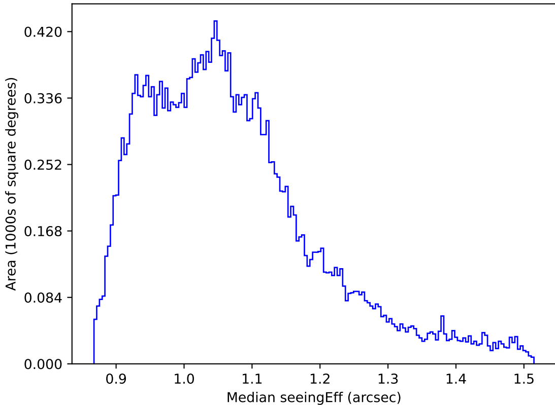
ddf_acor_sf10_lsf15_lsr10_v3.4_10yrs All sky r band: Median seeingEff
