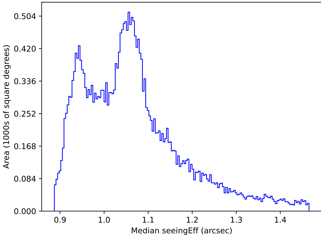
ddf_acor_sf10_lsf15_lsr10_v3.4_10yrs All sky all bands: Median seeingEff
