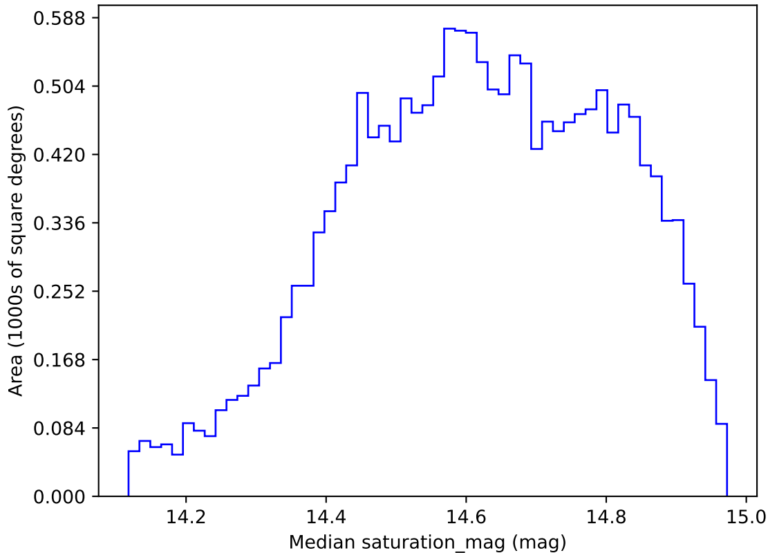
ddf_acor_sf10_lsf15_lsr10_v3.4_10yrs WFD r band: Median saturation_mag
