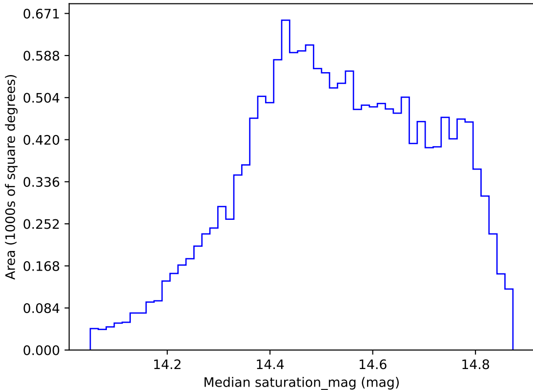
ddf_acor_sf10_lsf15_lsr10_v3.4_10yrs WFD i band: Median saturation_mag
