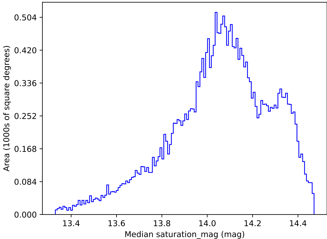
ddf_acor_sf10_lsf15_lsr10_v3.4_10yrs All sky z band: Median saturation_mag
