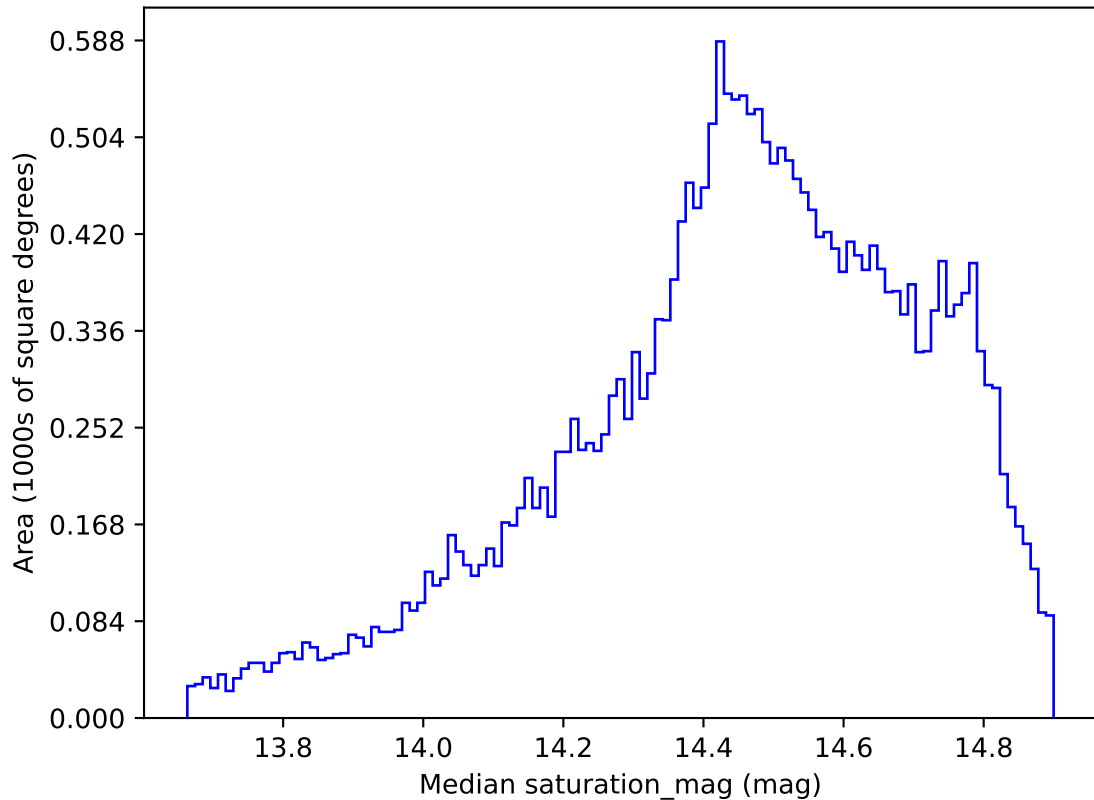
ddf_acor_sf10_lsf15_lsr10_v3.4_10yrs All sky i band: Median saturation_mag
