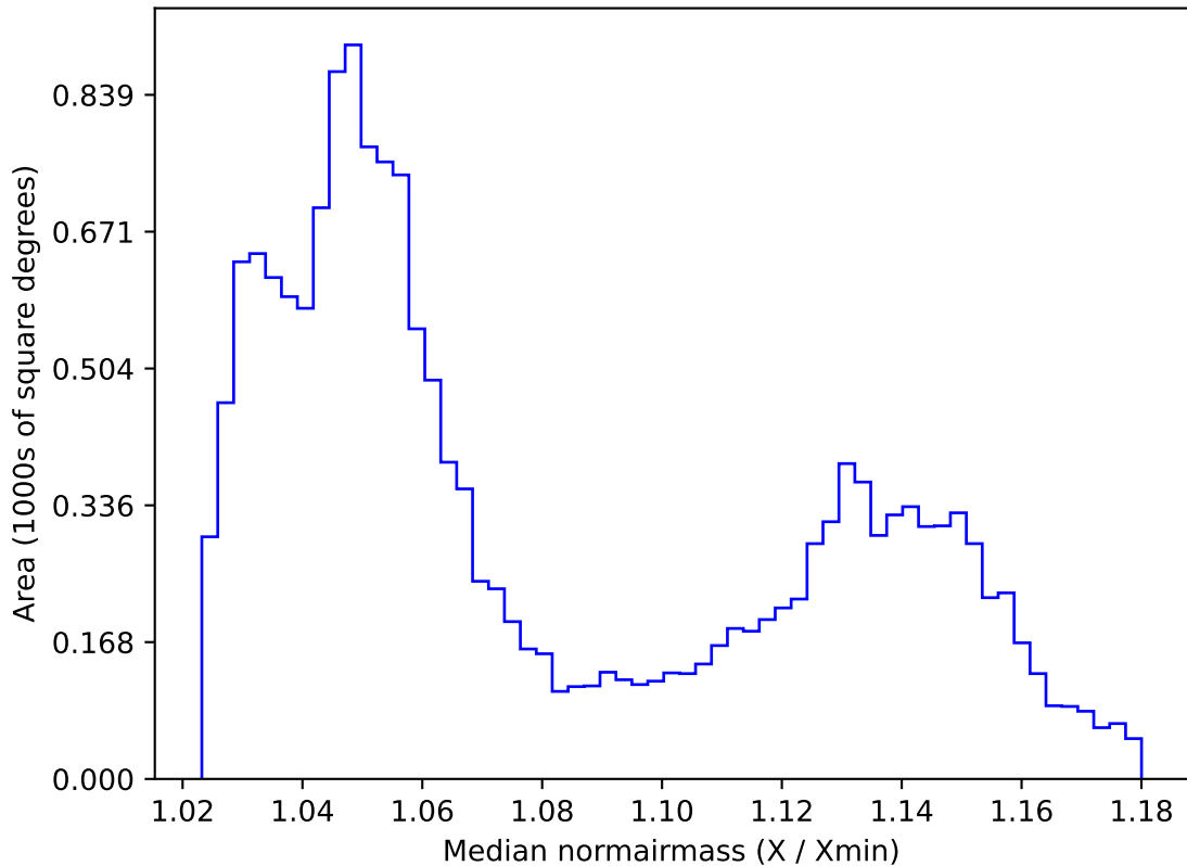
ddf_acor_sf10_lsf15_lsr10_v3.4_10yrs WFD all bands: Median normairmass
