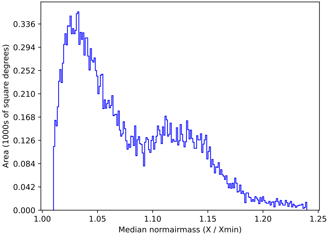
ddf_acor_sf10_ls15_lsr10_v3.4_10yrs All sky u band: Median normairmass
