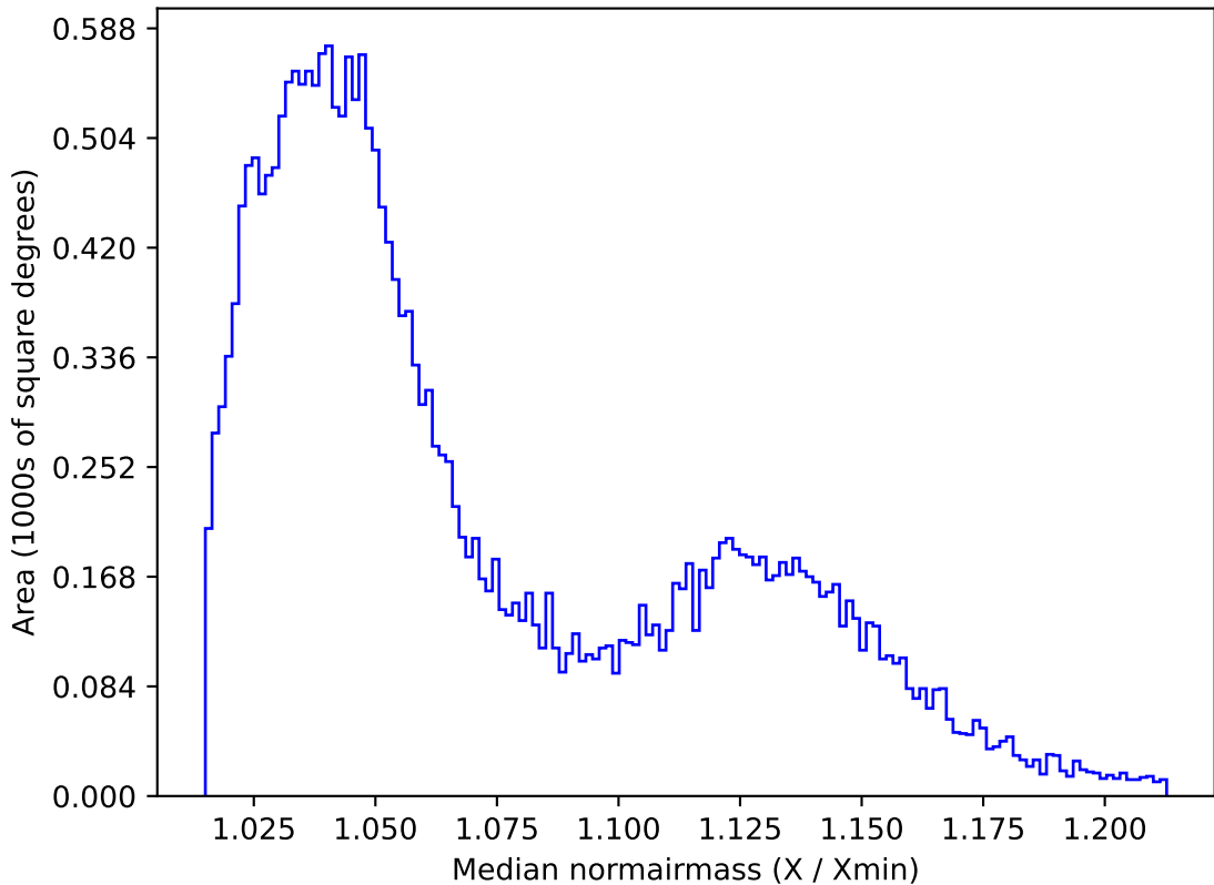
ddf_acor_sf10_lsf15_lsr10_v3.4_10yrs All sky r band: Median normairmass
