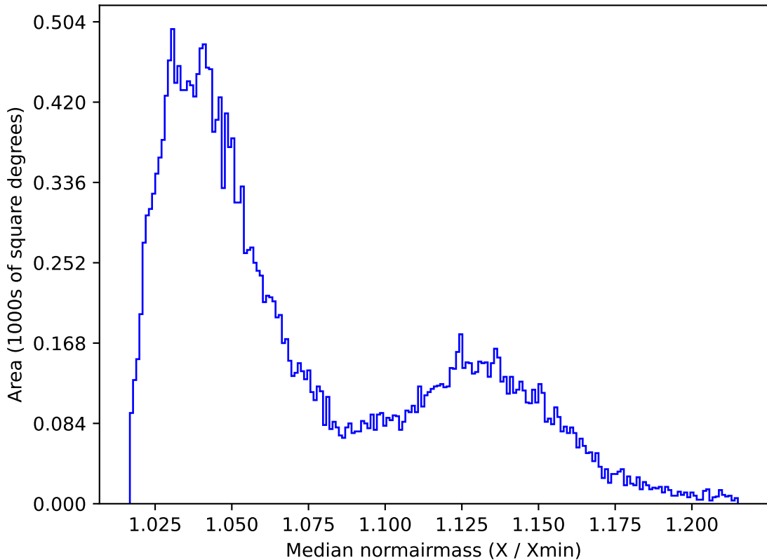
ddf_acor_sf10_lsf15_lsr10_v3.4_10yrs All sky i band: Median normairmass
