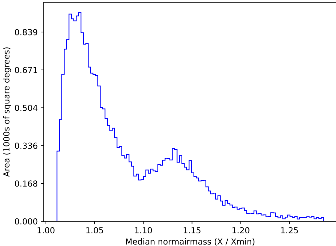
ddf_acor_sf10_ls15_lsr10_v3.4_10yrs All sky g band: Median normairmass
