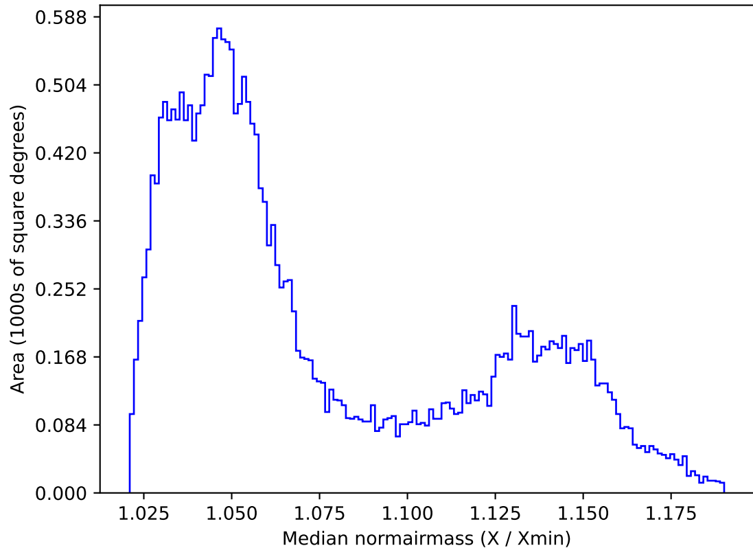
ddf_acor_sf10_lsf15_lsr10_v3.4_10yrs All sky all bands: Median normairmass
