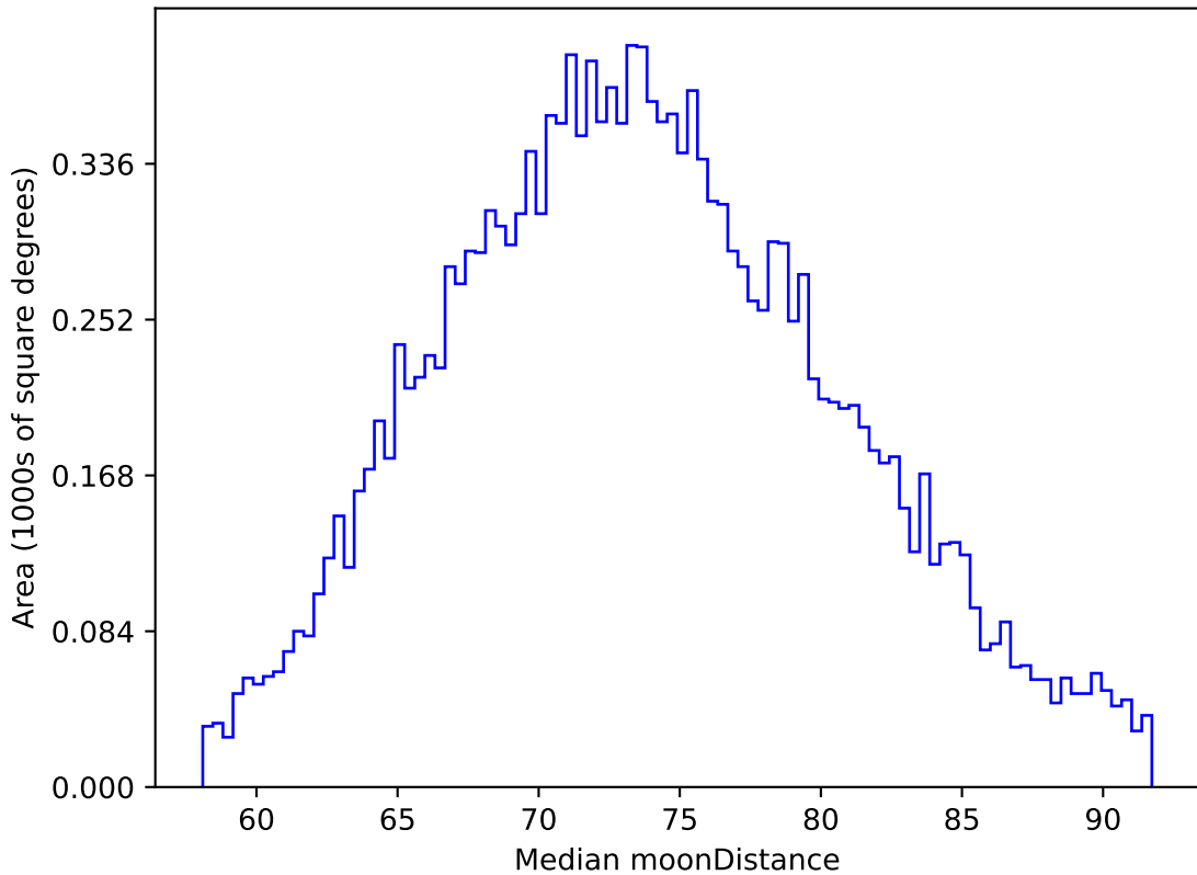
ddf_acor_sf10_lsf15_lsr10_v3.4_10yrs WFD z band: Median moonDistance
