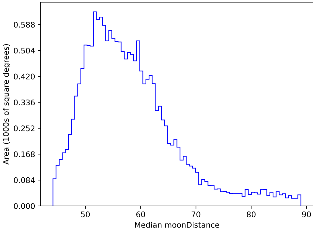
ddf_acor_sf10_lsf15_lsr10_v3.4_10yrs WFD y band: Median moonDistance
