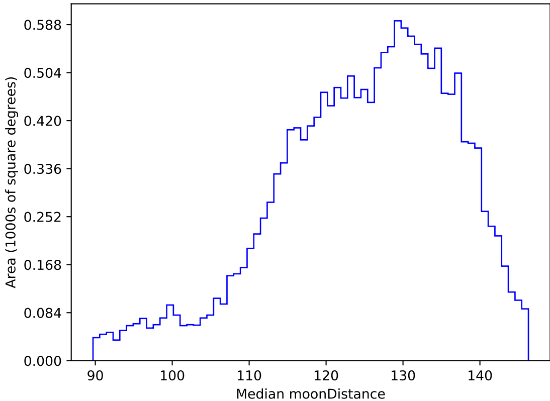
ddf_acor_sf10_lsf15_lsr10_v3.4_10yrs WFD u band: Median moonDistance
