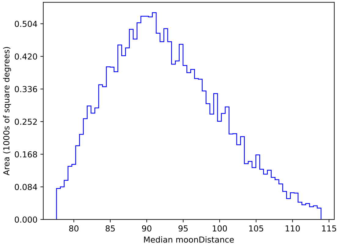
ddf_acor_sf10_lsf15_lsr10_v3.4_10yrs WFD i band: Median moonDistance
