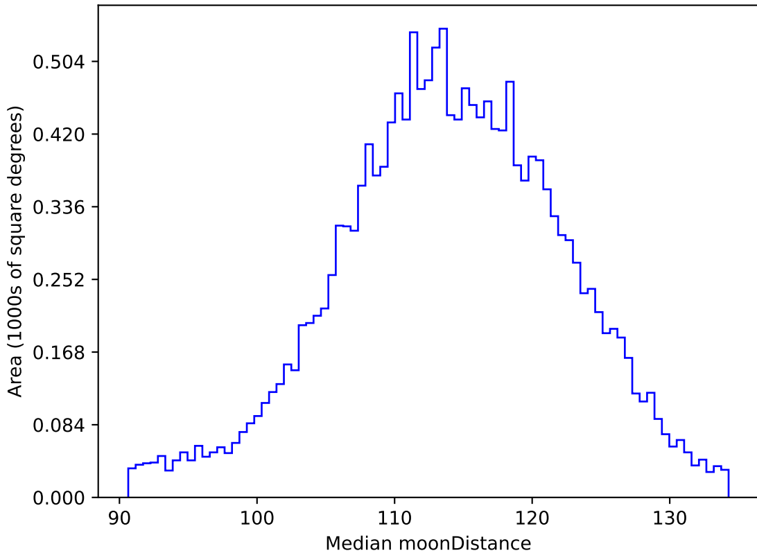
ddf_acor_sf10_ls15_lsr10_v3.4_10yrs WFD g band: Median moonDistance
