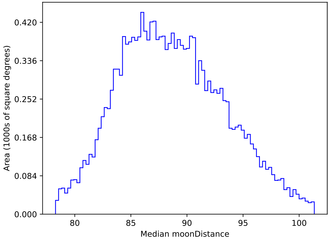
ddf_acor_sf10_lsf15_lsr10_v3.4_10yrs WFD all bands: Median moonDistance
