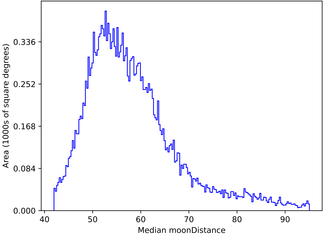
ddf_acor_sf10_lsf15_lsr10_v3.4_10yrs All sky y band: Median moonDistance
