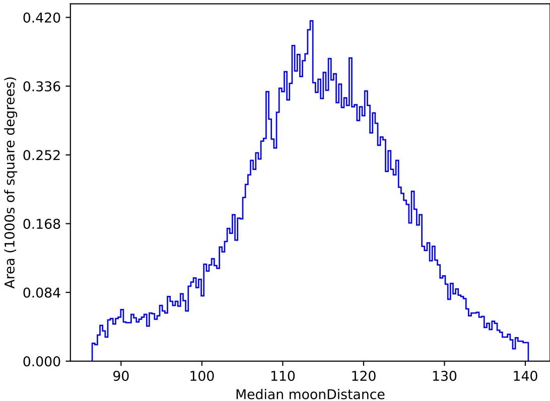
ddf_acor_sf10_lsf15_lsr10_v3.4_10yrs All sky g band: Median moonDistance
