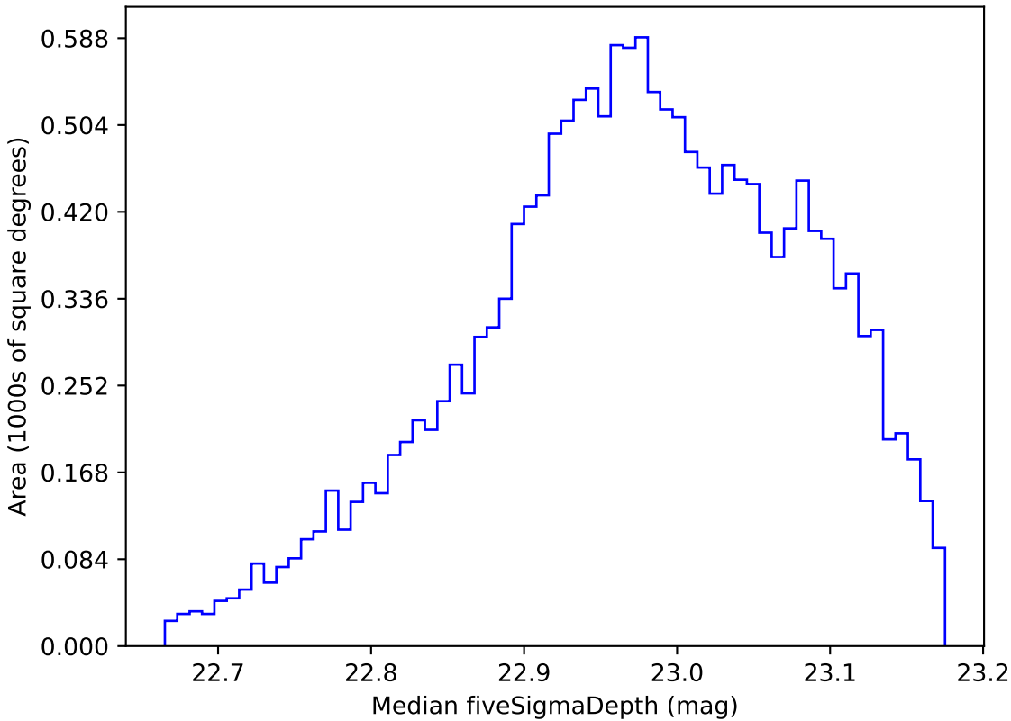
ddf_acor_sf10_lsf15_lsr10_v3.4_10yrs WFD z band: Median fiveSigmaDepth
