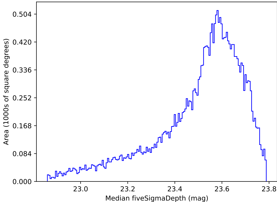
ddf_acor_sf10_lsf15_lsr10_v3.4_10yrs All sky i band: Median fiveSigmaDepth
