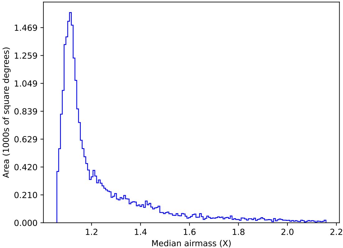
ddf_acor_sf10_lsf15_lsr10_v3.4_10yrs Yr 1 i band: Median airmass
