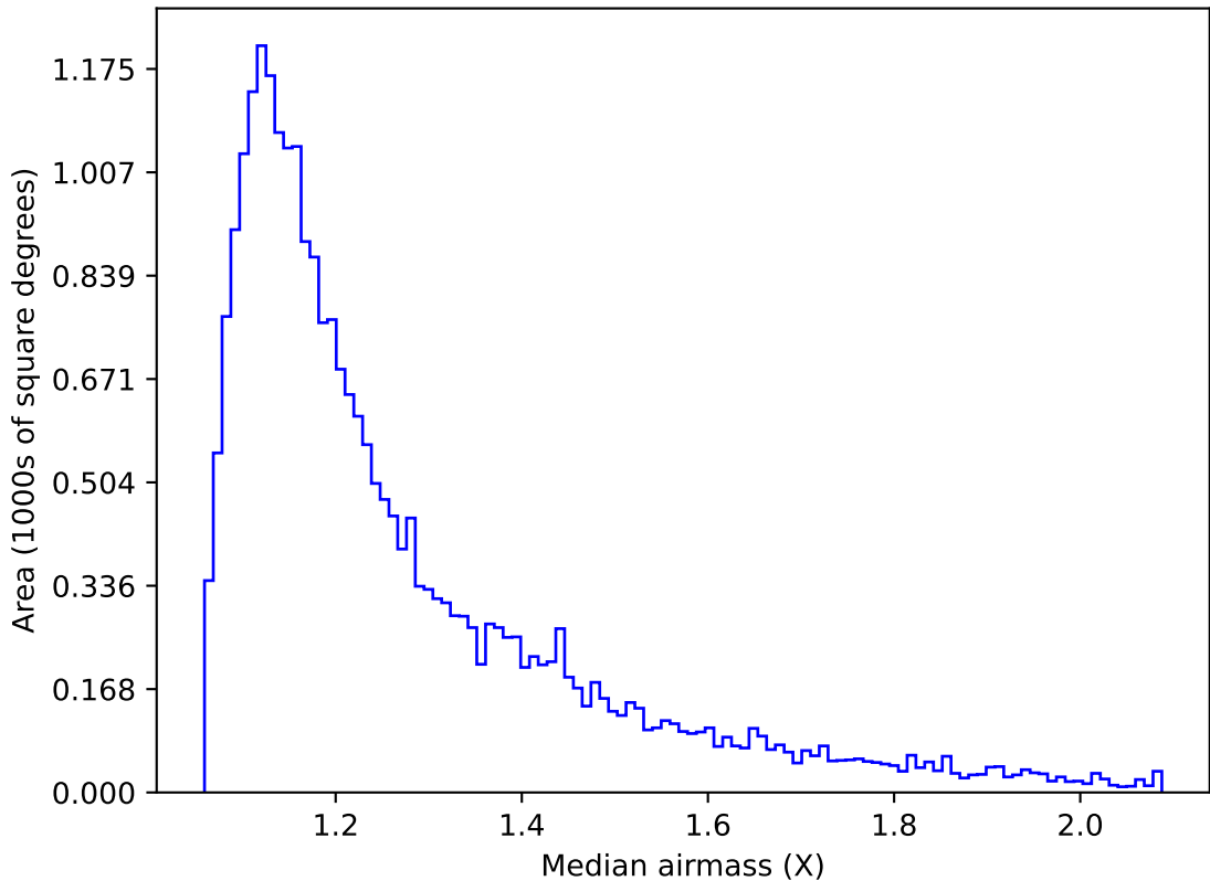
ddf_acor_sf10_lsf15_lsr10_v3.4_10yrs Yr 1 g band: Median airmass
