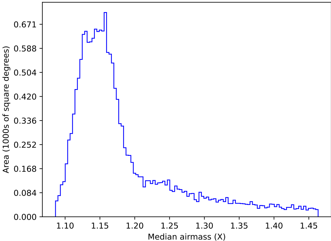
ddf_acor_sf10_lsf15_lsr10_v3.4_10yrs WFD z band: Median airmass
