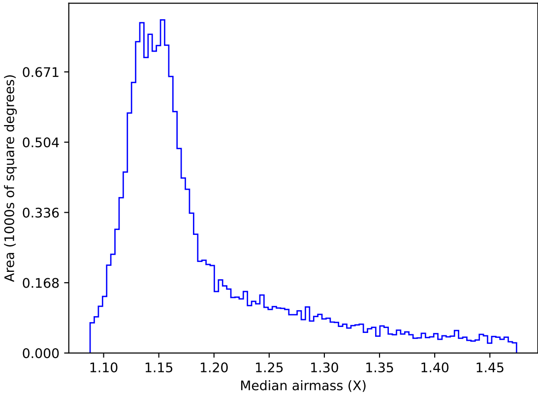
ddf_acor_sf10_ls15_lsr10_v3.4_10yrs WFD y band: Median airmass
