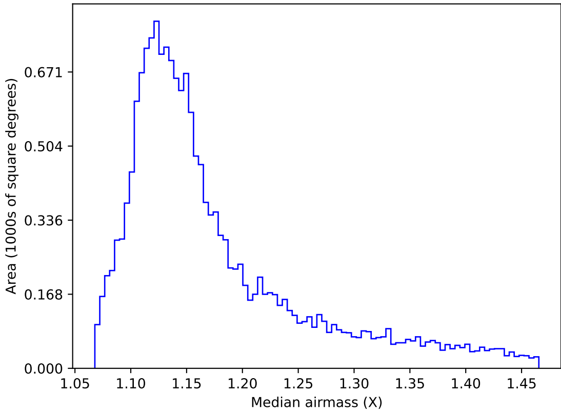
ddf_acor_sf10_ls15_lsr10_v3.4_10yrs WFD u band: Median airmass
