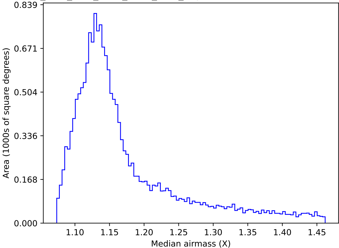
ddf_acor_sf10_lsf15_lsr10_v3.4_10yrs WFD r band: Median airmass
