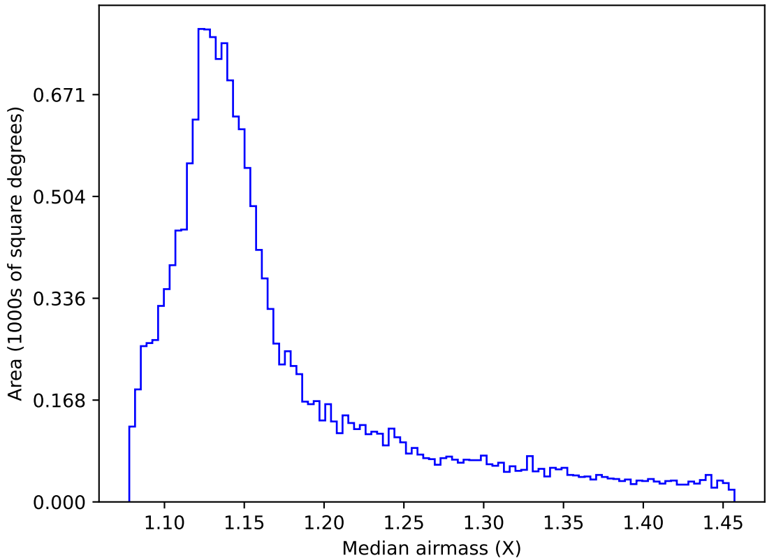
ddf_acor_sf10_lsf15_lsr10_v3.4_10yrs WFD i band: Median airmass
