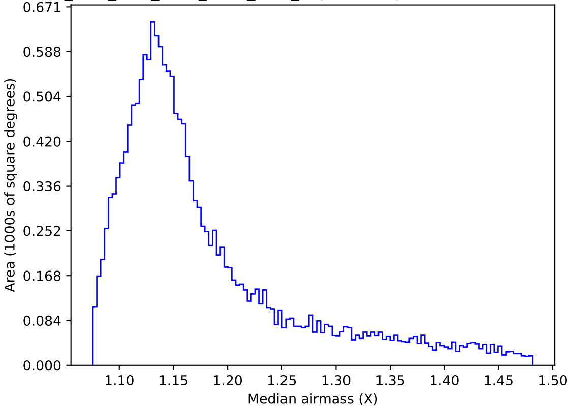
ddf_acor_sf10_ls15_lsr10_v3.4_10yrs WFD g band: Median airmass
