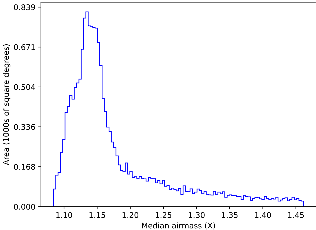
ddf_acor_sf10_lsf15_lsr10_v3.4_10yrs WFD all bands: Median airmass
