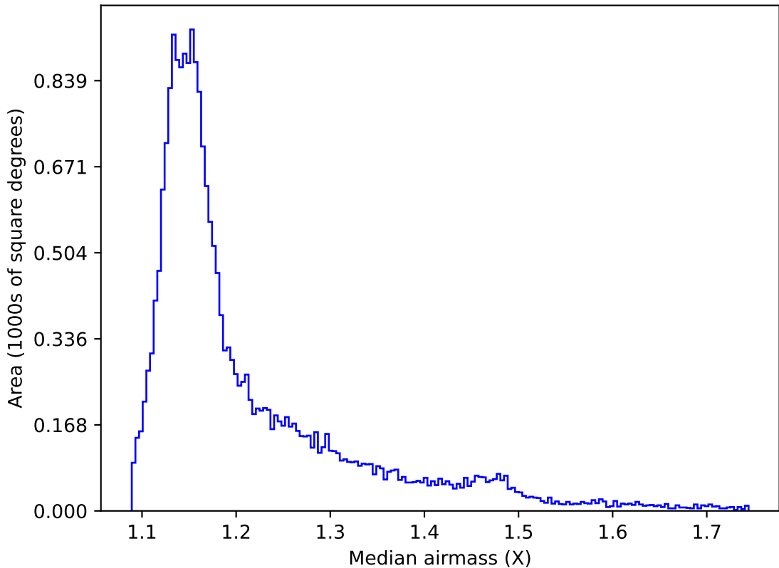
ddf_acor_sf10_lsf15_lsr10_v3.4_10yrs All sky y band: Median airmass
