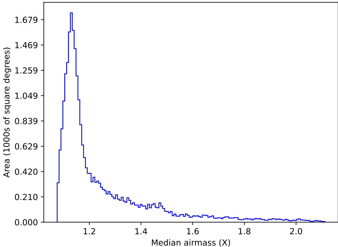
ddf_acor_sf10_lsf15_lsr10_v3.4_10yrs All sky r band: Median airmass
