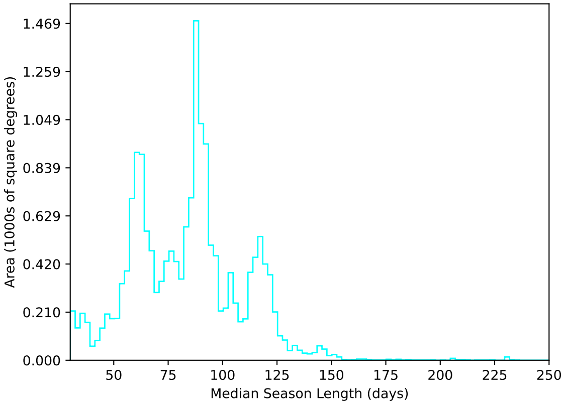
ddf_acor_sf10_ls15_lsr10_v3.4_10yrs WFD u band: Median Season Length
