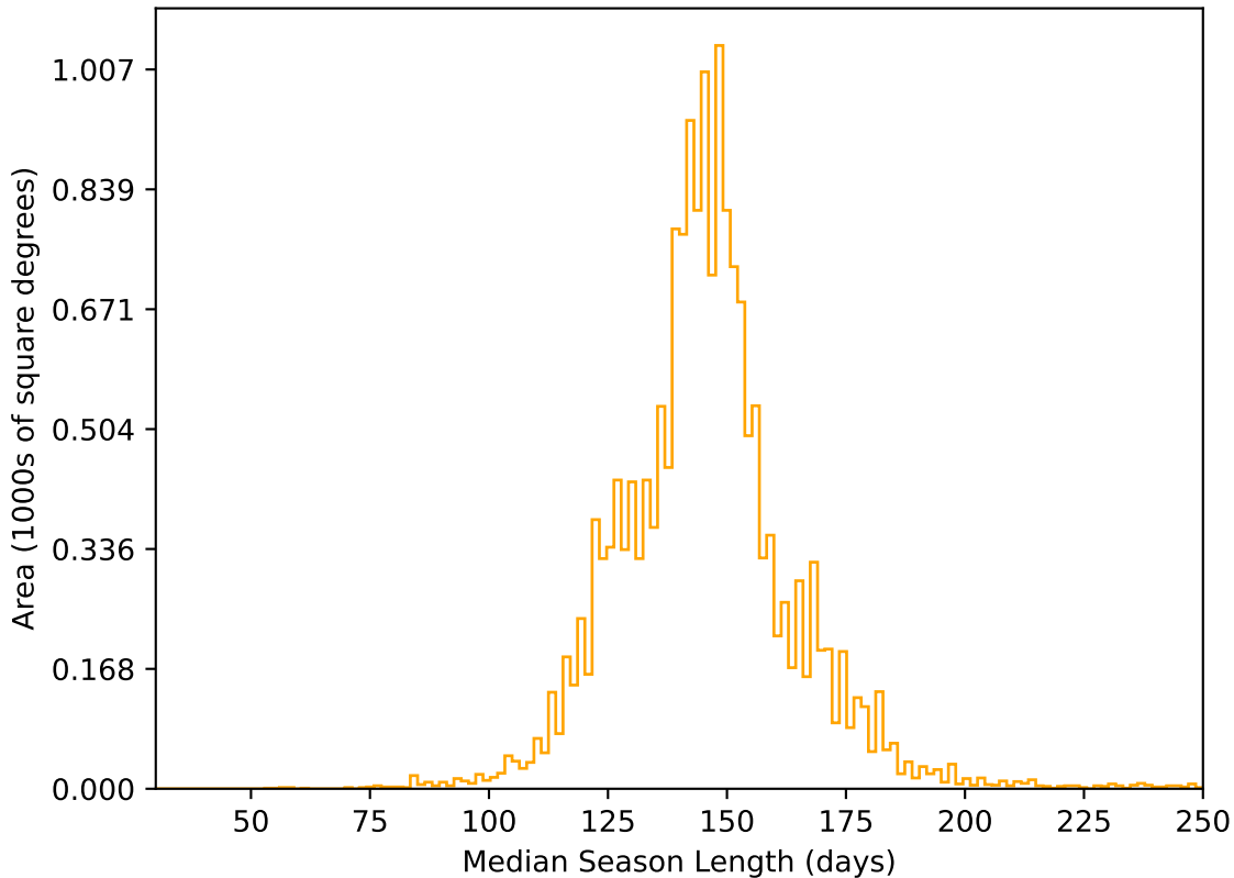
ddf_acor_sf10_lsf15_lsr10_v3.4_10yrs WFD r band: Median Season Length
